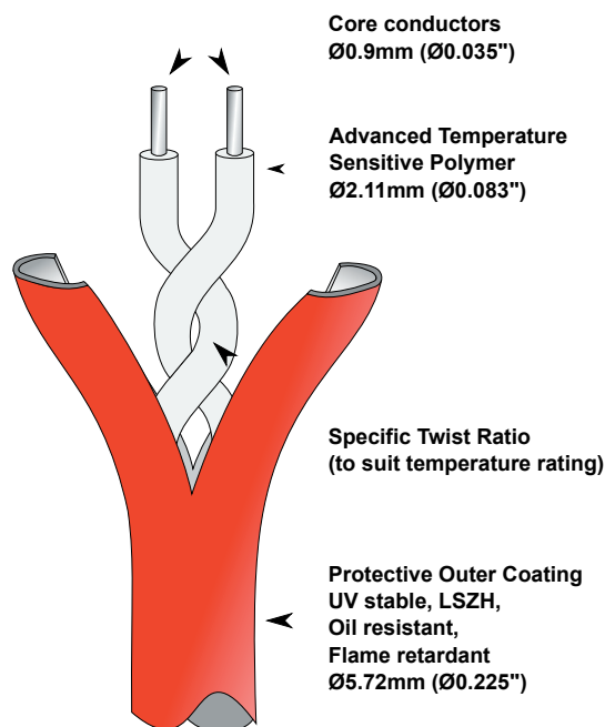
ProReact EN Digital Linear Heat Detection Cable Construction
